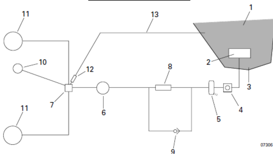
Figure 7.2: Fuel system
